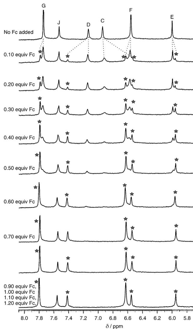
Figure 2. Partial 1 H NMR spectra (400 MHz, 50 mM NaCl + 10 mM borate buffer pH 8.9 in D 2 O) of host 1 (1.0 mM) in the presence of increasing concentrations of Fc . Proton resonances labeled with a star correspond to complexed 1 .
