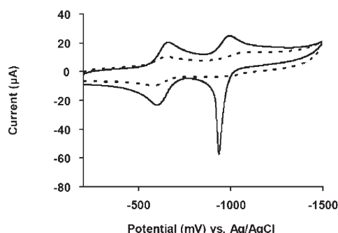
Figure 6. Cyclic voltammetric response on glassy carbon ( 0.071\text{ cm}^2 ) of 0.5\text{ mM MV}^{2+} in the absence (continuous line) and in the presence (discontinuous line) of 1.0\text{ mM 1} . The aqueous solution also contains 40\text{ mM NaCl} and 10\text{ mM sodium borate} (pH 8.9). Scan rate = 0.1\text{ V s}^{-1} .
