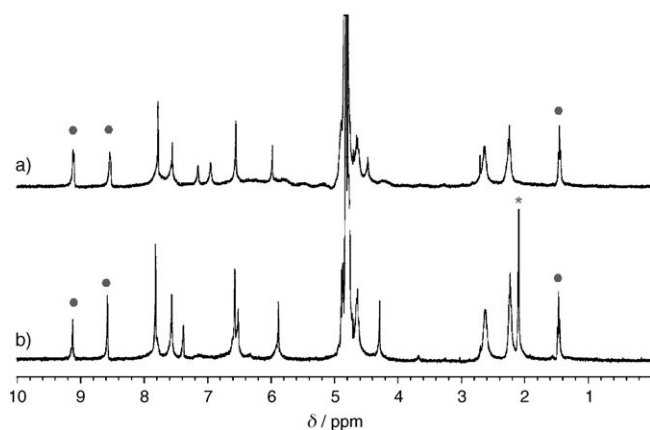
Figure 5. ^1\text{H} NMR spectra (400 MHz, 50 mm NaCl + 10 mm borate buffer pD=8.9 in \text{D}_2\text{O} ) of a) 2 mM \text{EV}^{2+} and 2 mM host 1 and b) 1 mM Fc , 2 mM \text{EV}^{2+} and 2 mM host 1 . The \text{EV}^{2+} protons are denoted by a circle and the encapsulated Fc protons by an asterisk.
