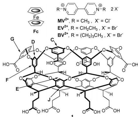
Figure 1. Structures of host 1 and the redox-active guests surveyed in this work
