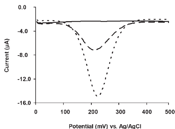
Figure 3. SWV response on a glassy carbon electrode ( 0.071 \text{ cm}^2 ) of 1.0 mM host 1 in 50 mM NaCl + 10 mM pH 8.9 borate buffer in the presence of 0.5 equiv (continuous line), 1.0 equiv (discontinuous line) and 2.0 equiv (dotted line) guest Fc . Scan rate: 0.1 \text{ V s}^{-1} .
